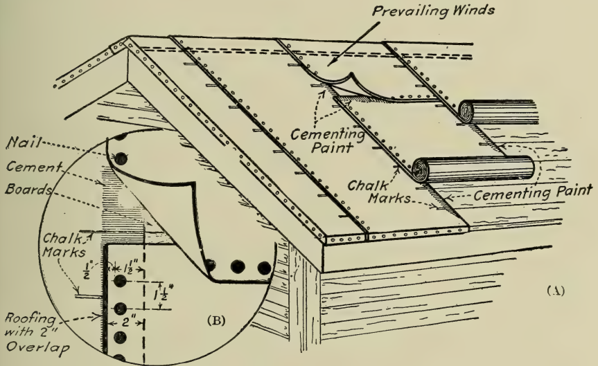
FIG. 143.—Laying Roll Roofing in Single Course.
